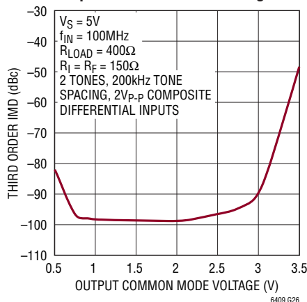
Intermodulation Distortion vs Output Common Mode Voltage
