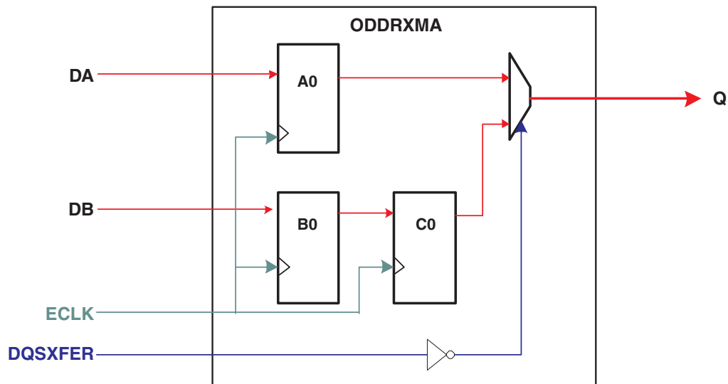
Figure 12-17. Output Register Block in ODDR X MA Mode
