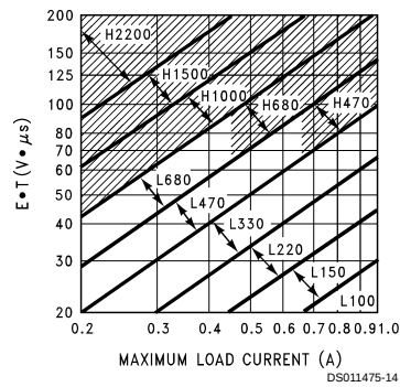
FIGURE 7. LM2575(HV)-ADJ
