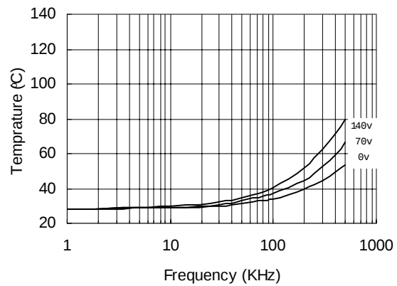
Figure 22. IR2183 vs. Frequency (IRFBC20), R_{gate} \approx 33\Omega , V_{CC} = 15V
