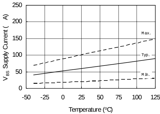
Figure 14A. V_{BS} Supply Current vs. Temperature
