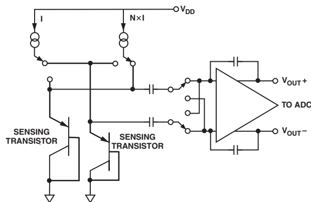
Figure 3. Temperature Measurement Technique
