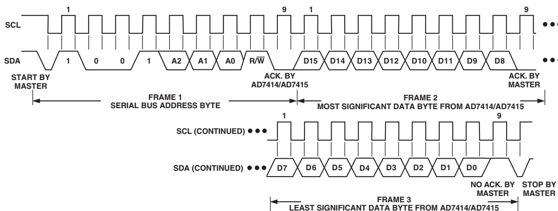
Figure 9. Reading Two Bytes of Data from the Temperature Value Register
