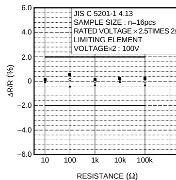
Fig.4 Overload
