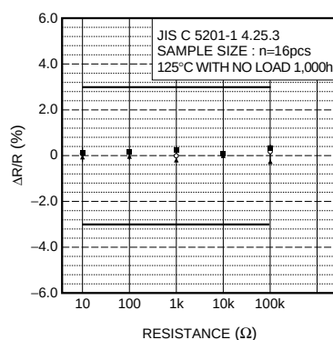
Fig.9 Endurance
