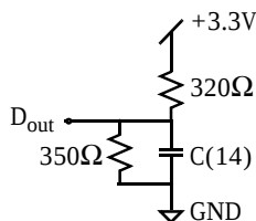
Figure C: Output load
