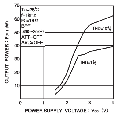
Fig.10 Output power vs. power supply voltage
