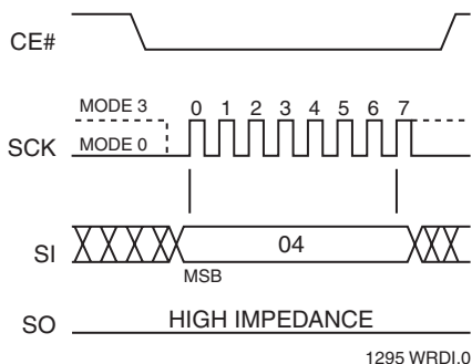
FIGURE 18: Write Disable (WRDI) Sequence
