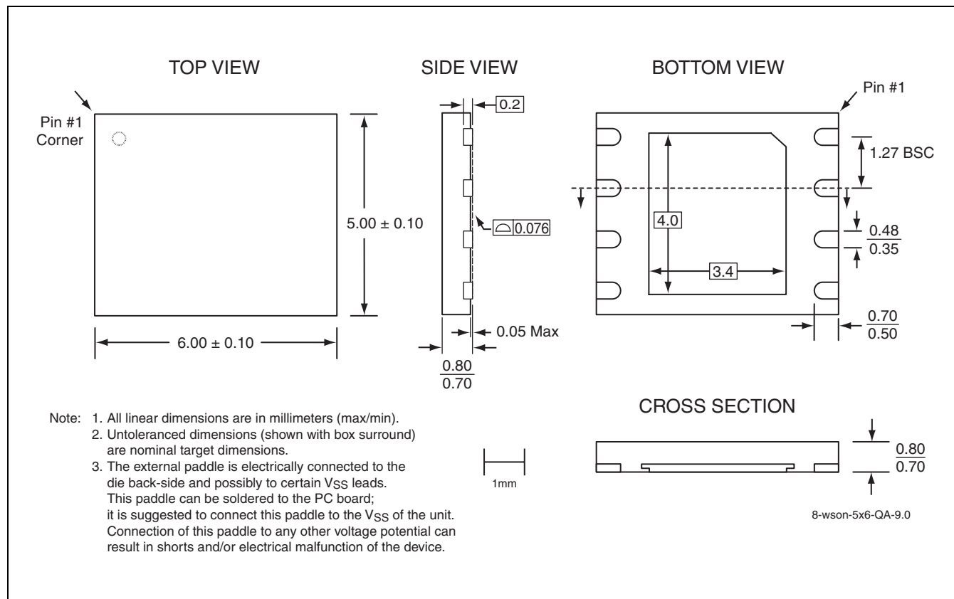
FIGURE 30: 8-Contact Very-very-thin Small Outline No-lead (WSO) SST Package Code: QA
