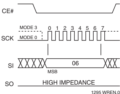
FIGURE 17: Write Enable (WREN) Sequence
