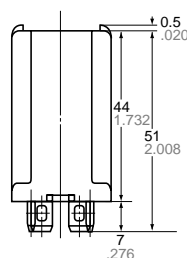
External dimensions
