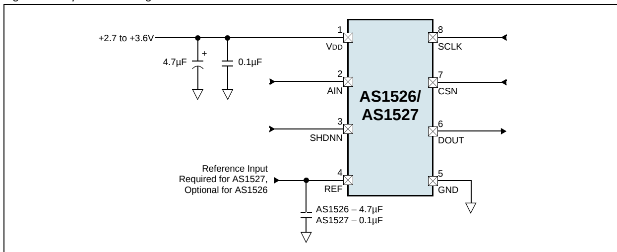
Figure 23. Operational Diagram
