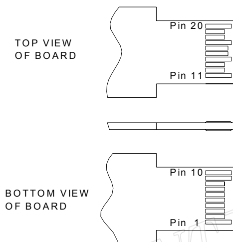
Figure 4, Pin View
