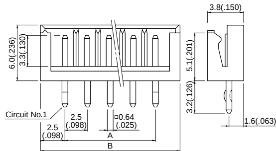
(3 to 15 circuits)
