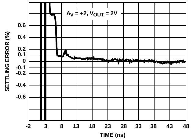
FIGURE 22. SETTLING RESPONSE
