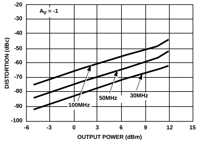
FIGURE 32. THIRD HARMONIC DISTORTION vs P_{\text{OUT}}
