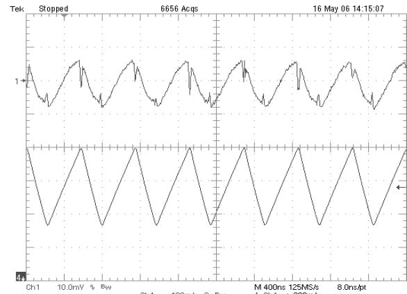
Figure 12. Negative Output Voltage Ripple in CCM 1 V_{OUTN} , 10 mV/div AC, 4 I_{LN} , 100 mA/div DC, I_{OUTN} = 100 mA
