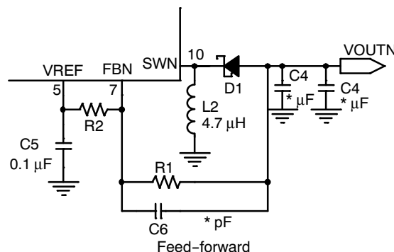
Figure 15. Inverter Compensation
