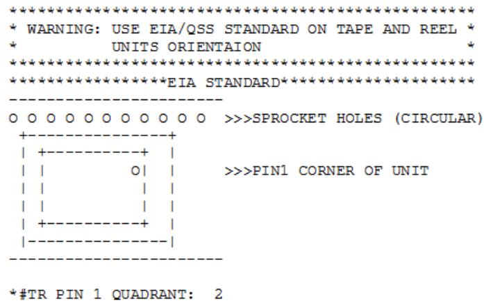
Figure A-6. Tape and Reel QFP Pin 1 Location
