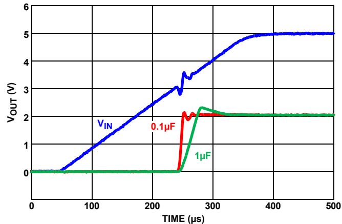
FIGURE 63. TURN-ON TIME
