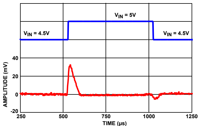
FIGURE 59. LINE TRANSIENT RESPONSE WITH 10μF LOAD
