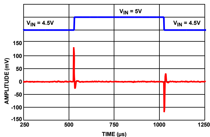
FIGURE 58. LINE TRANSIENT RESPONSE WITH 0.1μF LOAD
