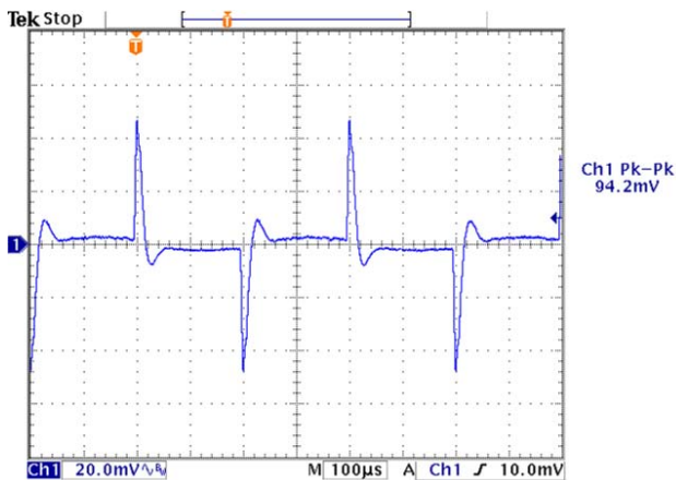
Figure 21. Transient Response without Optimal Voltage Positioning
