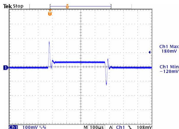
Figure 14. V_{in}=12V , V_{out}=1.0V
