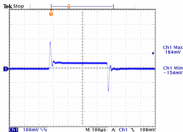
Figure 13. V_{in}=12V , V_{out}=2.5V
