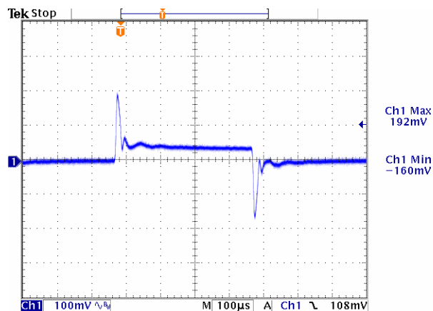
Figure 12. V_{in}=12V , V_{out}=5.0V
