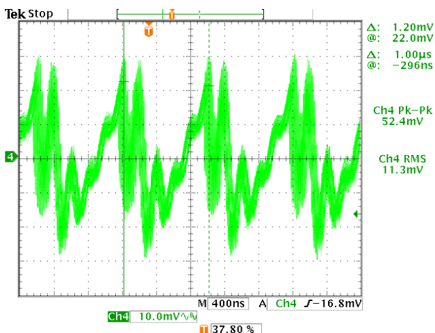
Figure 40. Input Voltage Noise, No Interleave
