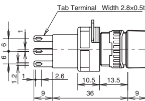
Solder/Tab Terminal
