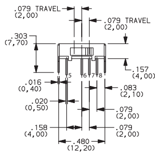
OS203011MA2QP1 DP3T
