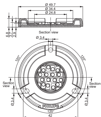
Lexel LED SLM 800 25W/RGB 20mm
