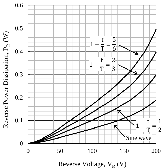
Figure 3-5 P_R - V_R
