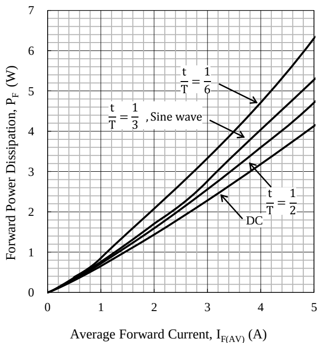
Figure 3-4 P_F - I_{F(AV)}
