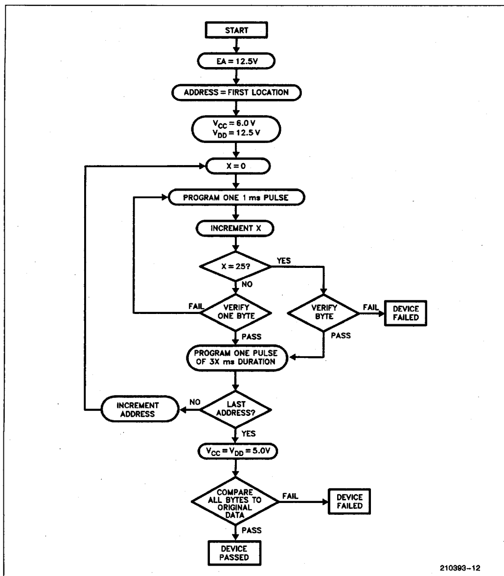
Figure 9. Programming Algorithm
