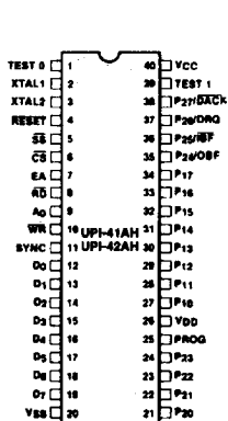
Figure 1. DIP Pin Configuration
