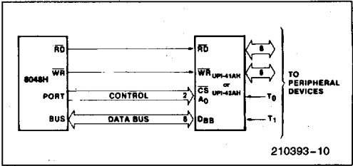
Figure 6. 8048H-UPI-41/42 Interface
