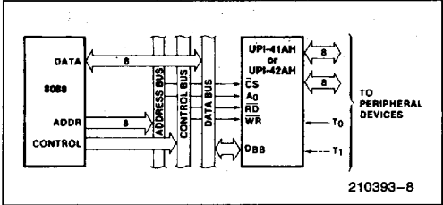
Figure 5. 8088-UPI-41AH/42AH Interface
