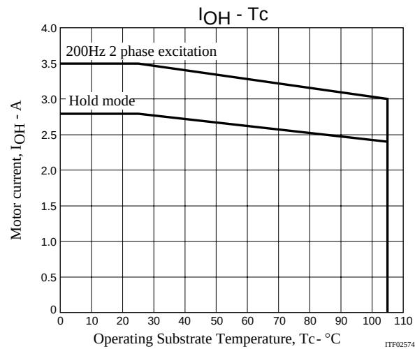
Derating Curve of Motor Current, I_{OH} , vs. STK672-440A-E Operating Substrate Temperature, T_c
