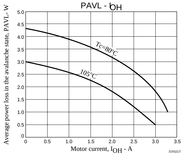
Figure 3 Allowable Loss Range, PAVL - I_{OH} During STK672-440A-E Avalanche Operations
