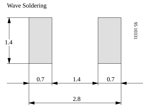
Figure 13. Recommended foot pads (in mm)
