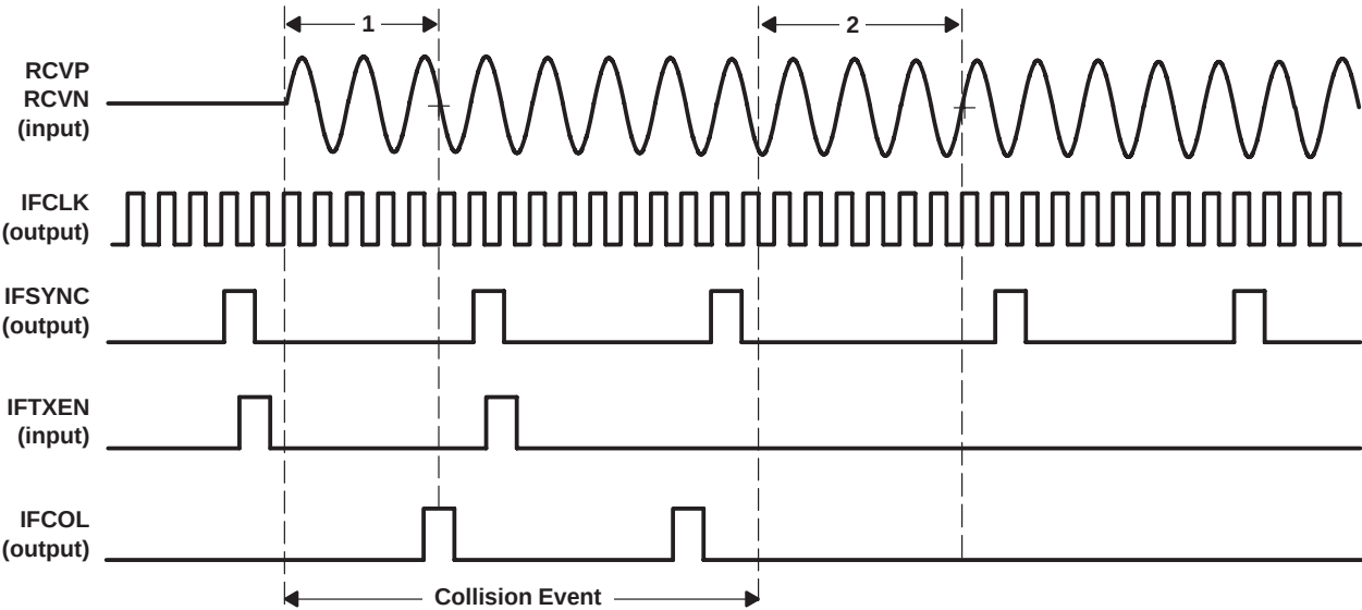
Figure 17. Collision Detect
