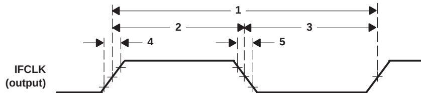
Figure 11. Clock Limits
