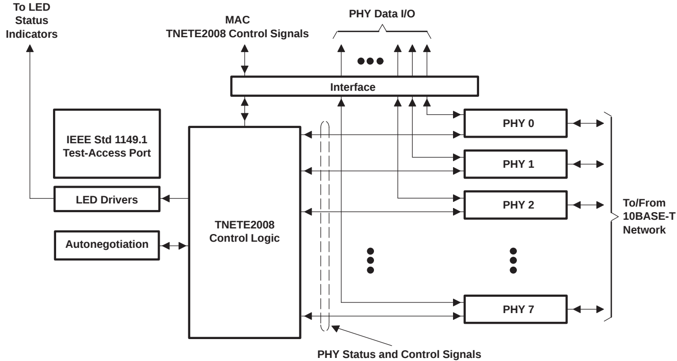
Figure 1. OctalPHY Architecture
