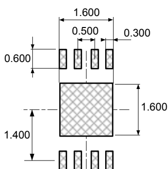
Figure 27. UDFPN8 - Recommended footprint
