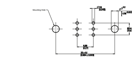
Shell Size Contact Arrangement No. of Size 20 Cavities No. of Size 8 Cavities E 2W2/2WK2 0 #20 2 #8
