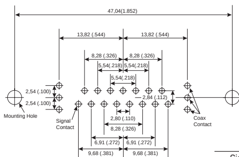
Shell Size Contact Arrangement No. of Size 20 Cavities No. of Size 8 Cavities B 17W2 15 #20 2 #8
