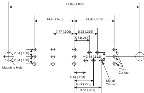
Shell Size Contact Arrangement No. of Size 20 Cavities No. of Size 8 Cavities B 9W4 5 #20 4 #8
