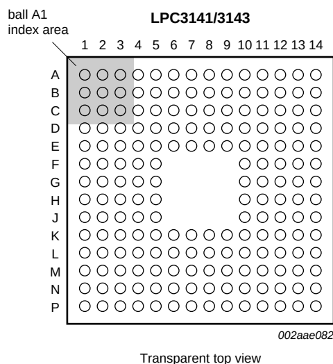
Fig 2. LPC3141/3143 pinning TFBGA180 package
