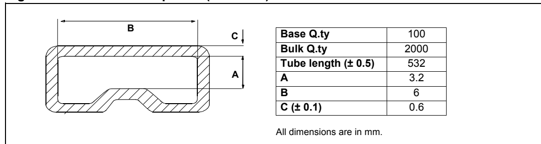
Figure 36. SO-8 tube shipment (no suffix)
