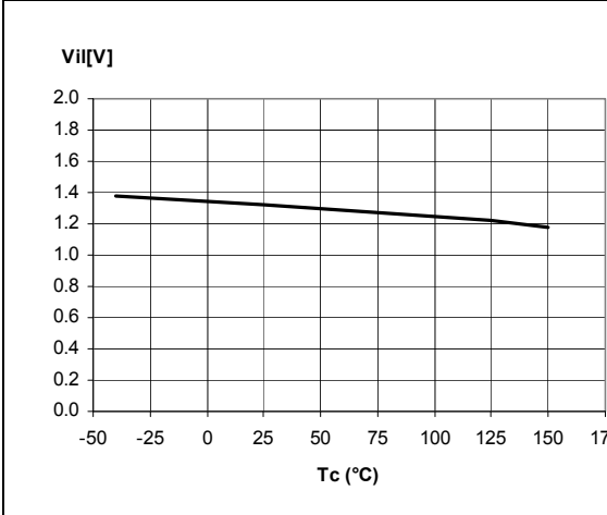
Figure 12. Input low-level voltage
