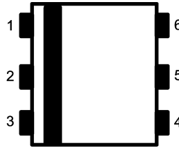
Figure 2. SOT23-6, Top View
