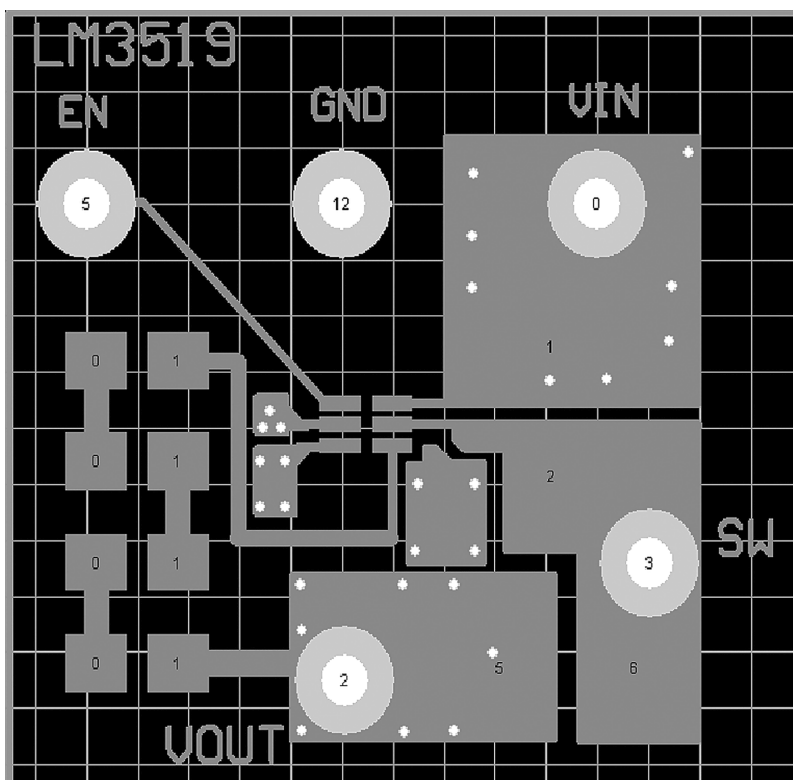
Figure 3. Top Layer
