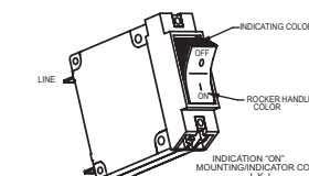
MARKING DETAIL "A" (SEE TABLE)
