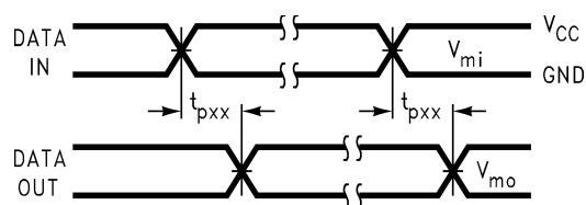
FIGURE 8. Waveform for Inverting and Non-inverting Functions
