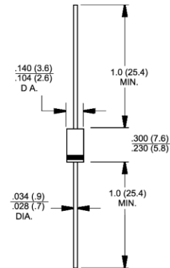
DO-204AC (DO-15)
