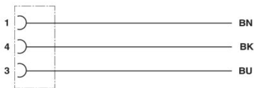
Contact assignment of the M12 socket
