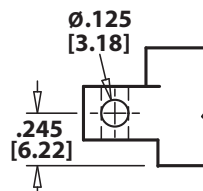
SIDE MOUNTING (S)
