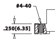
FLUSH MOUNTING WITH THREADED INSERT (T)
