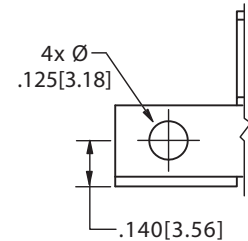
FLUSH, SIDE MOUNTING with CLEARANCE HOLES (Z)
