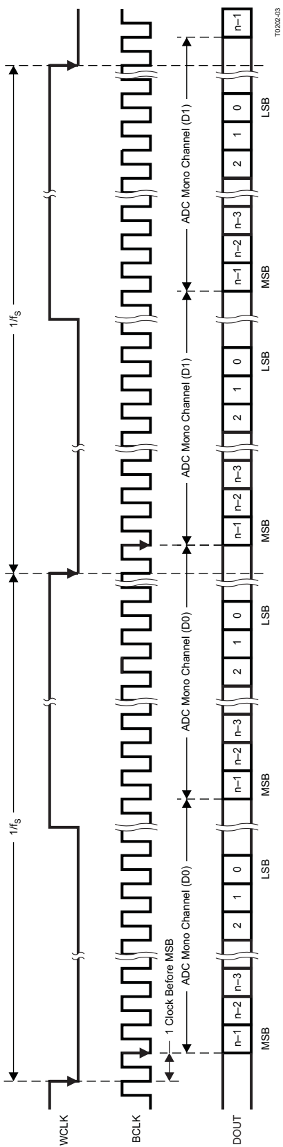
Figure 7-44. Timing Diagram for I²S Mode for Mono Audio ADC
