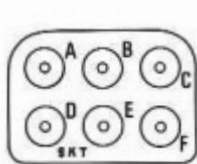
Layout 06 6 Size 20 Contacts
