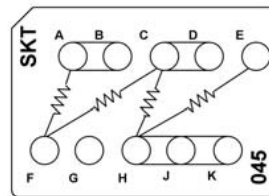
CTJ420E045 Two 40 k \Omega Resistors, 1/10 W Two 50 k \Omega Resistors, 1/10 W
