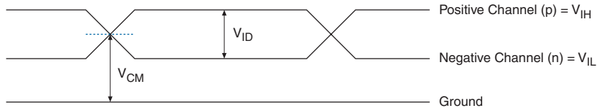
Figure 4–5. Receiver Input Waveforms for Differential I/O Standards
