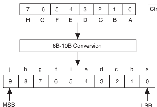
Figure 2–6. 8B/10B Encoder
