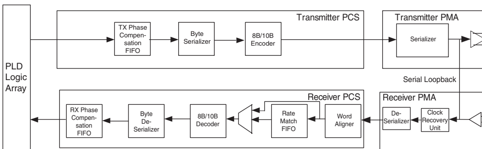
Figure 2–13. Transceiver Data Path in Serial Loopback
