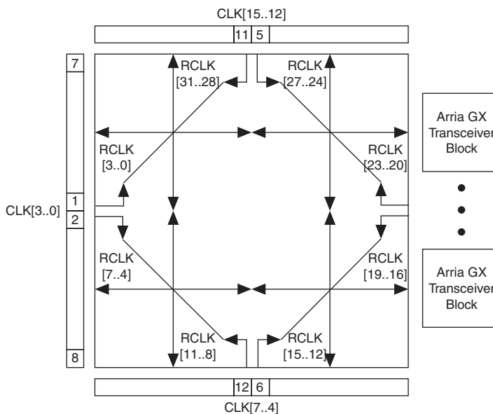
Figure 2–17. Regional Clock Resources in Arria GX
