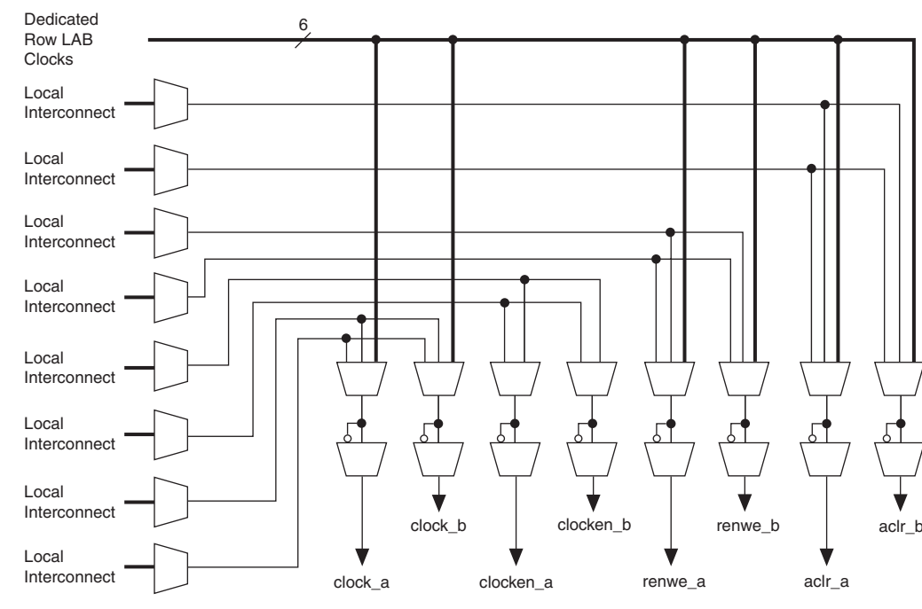
Figure 2-37. M4K RAM Block Control Signals
