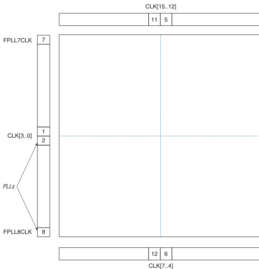
Figure 2–54. PLL Locations
