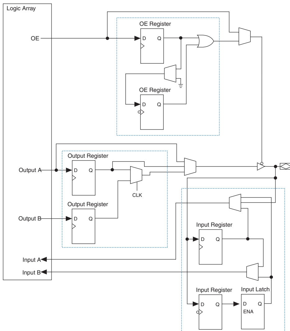
Figure 2–60. Arria GX IOE Structure
