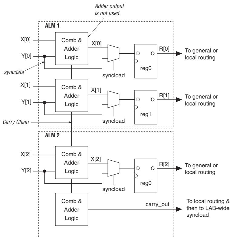
Figure 2–28. Conditional Operation Example
