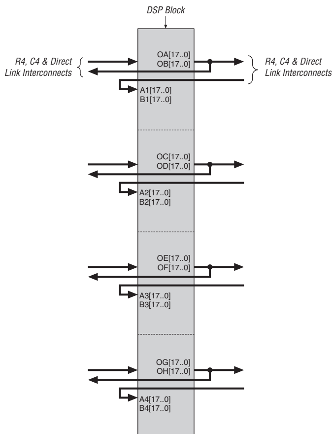
Figure 2–45. DSP Block Interconnect Interface
