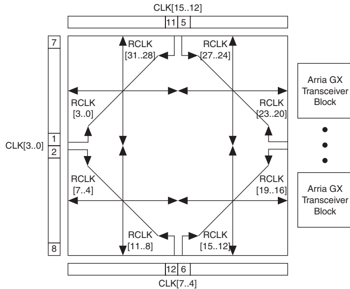
Figure 2–48. Regional Clocks
