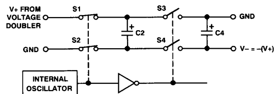
Figure 2. Voltage Inverter
