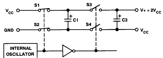
Figure 1. Voltage Doubler
