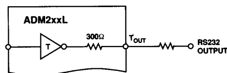
Figure 3. Resistor Protection to \pm 20\text{ V} for Transmitter Outputs
