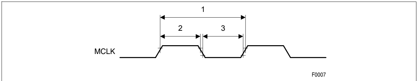
Figure 48 MCLK Timing
