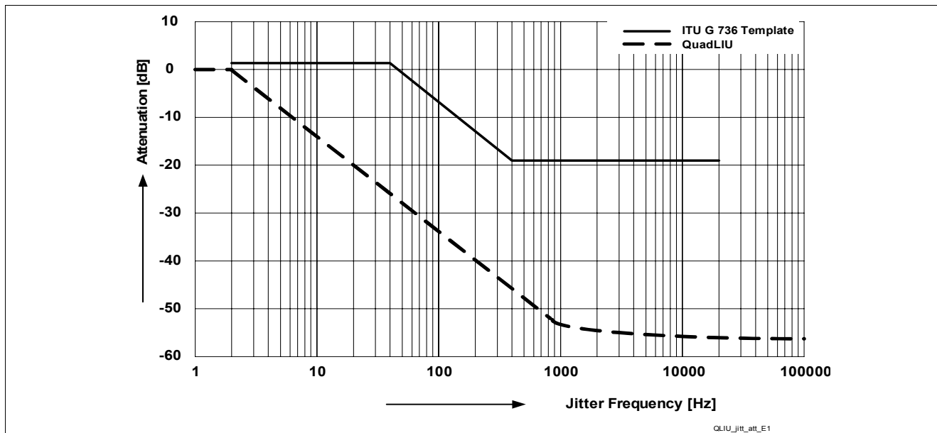
Figure 30 Jitter Attenuation Performance (E1)
