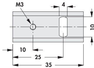
11 K/W TO 220
