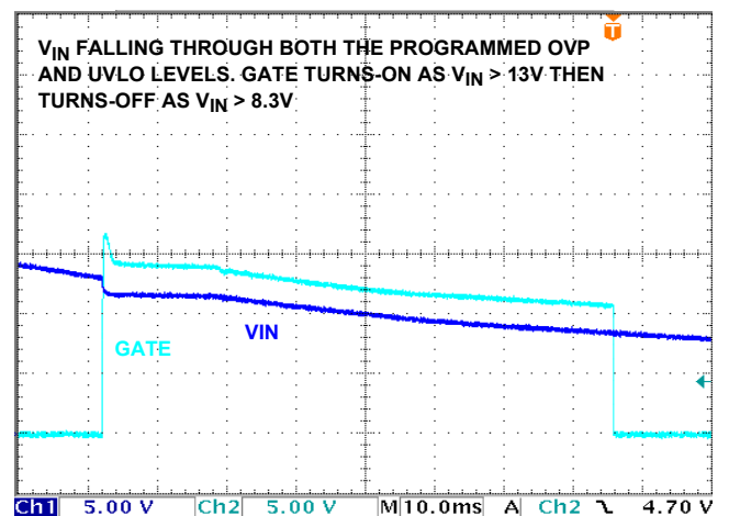
FIGURE 32. ISL6146C FALLING, V_{IN} OVP AND UVLO FUNCTION
