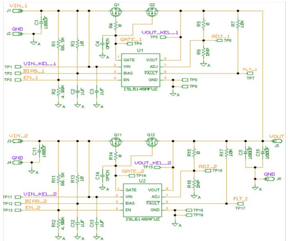
FIGURE 57. ISL6146AEVAL1Z SCHEMATIC
