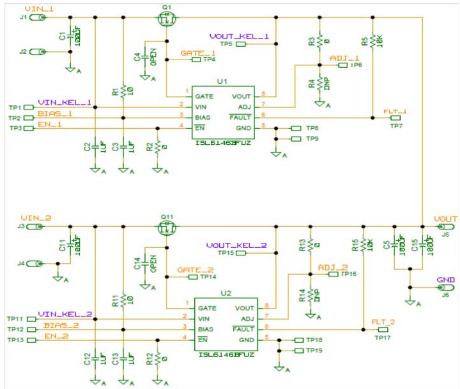
FIGURE 59. ISL6146BEVAL1Z SCHEMATIC
