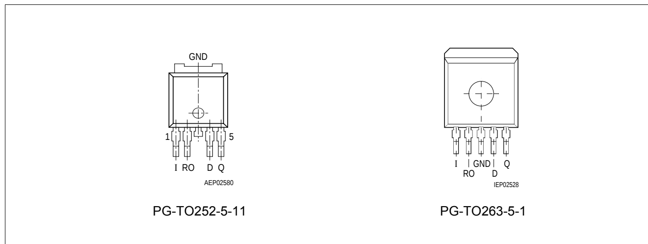
Figure 2 Pin Assignment
