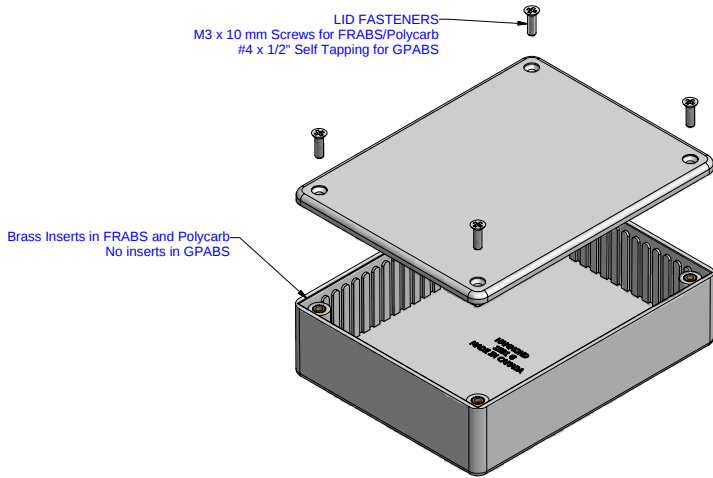
EXPLODED VIEW OF ENCLOSURE
