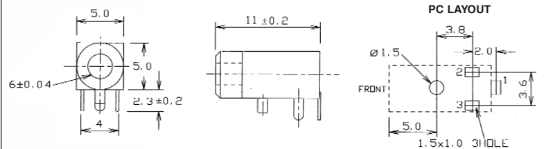
JYO-29 mono switched low profile 2.5mm Jack Socket. Right Angle PCB mounting.
