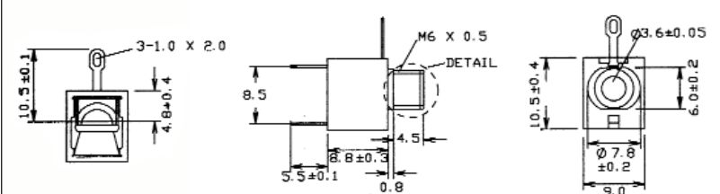
JYO-35 mono switched 3.5mm Jack Socket. Panel mounting with solder tags. Supplied with ring nut.
