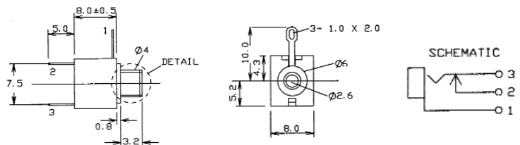
JYO-25 mono switched 2.5mm Jack Socket. Panel mounting with solder tags. Supplied with ring nut.
