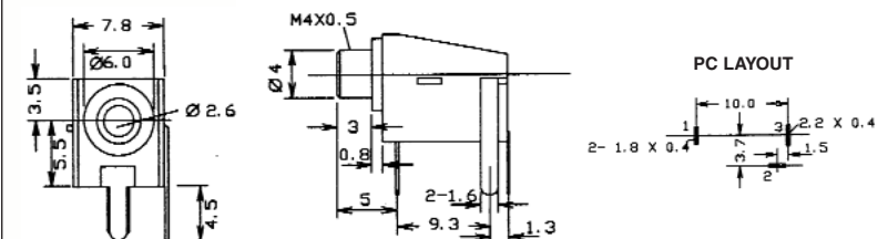
JYO-26 mono switched 2.5mm Jack. Right Angle PCB mounting with ring nut. Thread-less nose version JYO-26A.
