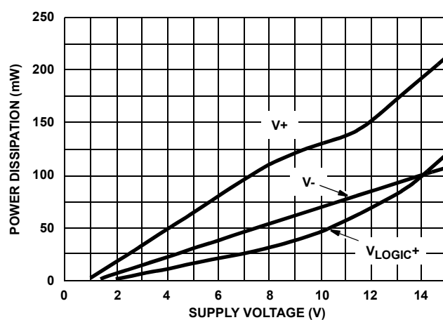
FIGURE 9. POWER DISSIPATION vs SUPPLY VOLTAGE (NO LOAD CONDITION)
