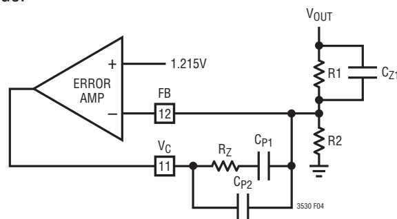
Figure 5. Error Amplifier with Type III Compensation
