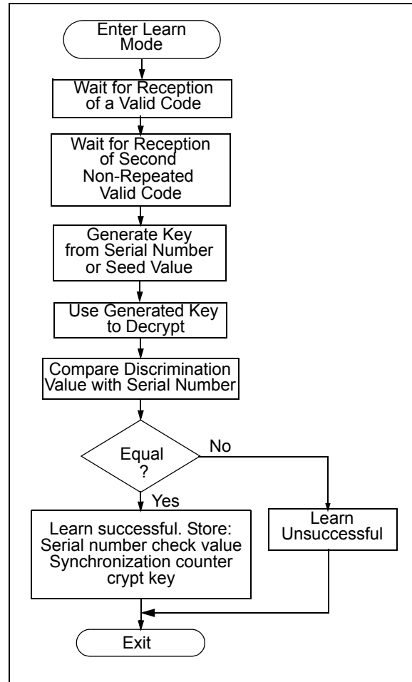
FIGURE 4-1: LEARN SEQUENCE
