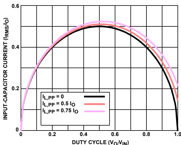
FIGURE 25. NORMALIZED INPUT-CAPACITOR RMS CURRENT vs DUTY CYCLE FOR SINGLE-PHASE CONVERTER
